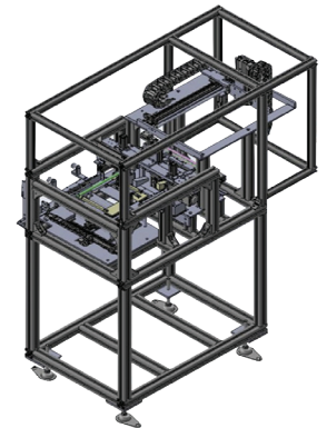
Transferring Machine
