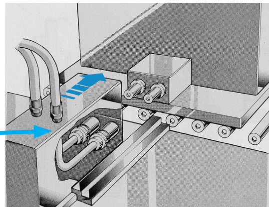
Oil and air circuits single action connect/disconnect for automated mold replacement
